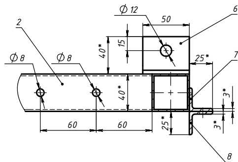
K-K (1:2)
