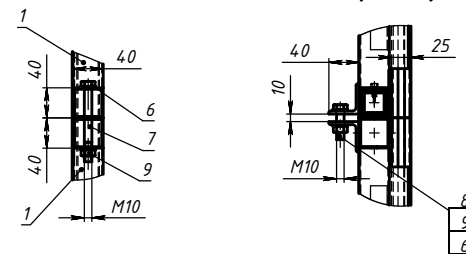
E-E (1:5)
